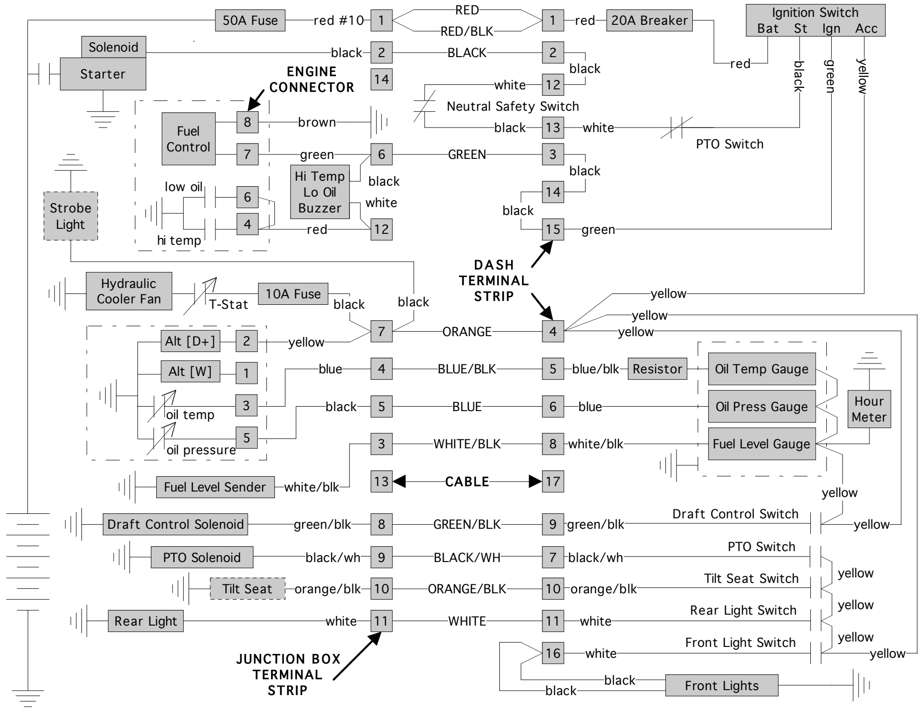
PT1845 Wiring Logic Diagram derived from Power Trac drawings E463x4 and E495 7/27/03 [rev 8/2/03 jhc]
